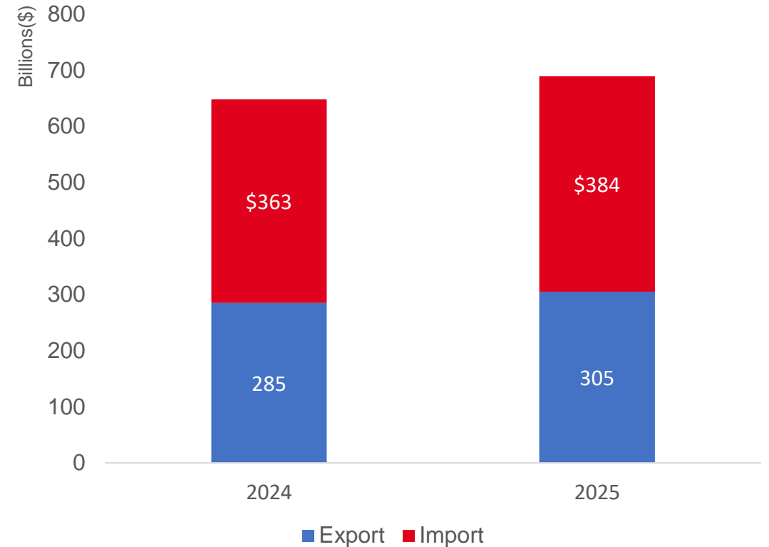
Foreign Trade Growth Estimate, 2024-2025
